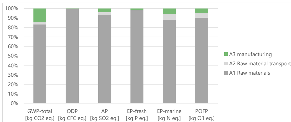
Figure 2: Cradle-to-Gate Impacts for Electrical Metallic Tubing, Rochelle, IL (Average EAF Steel Supply Mix)
